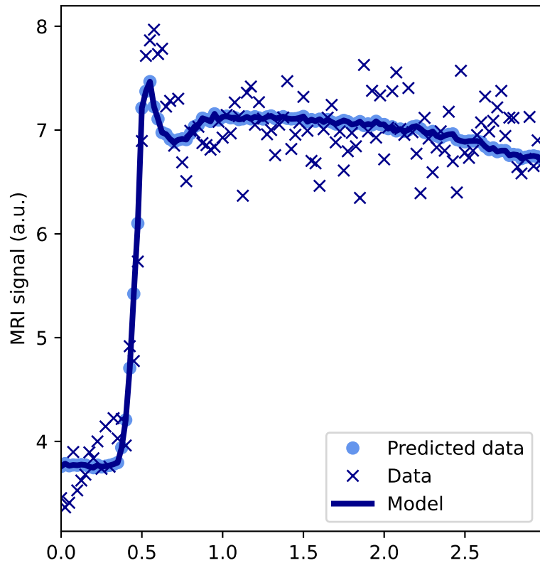
MRI signals
